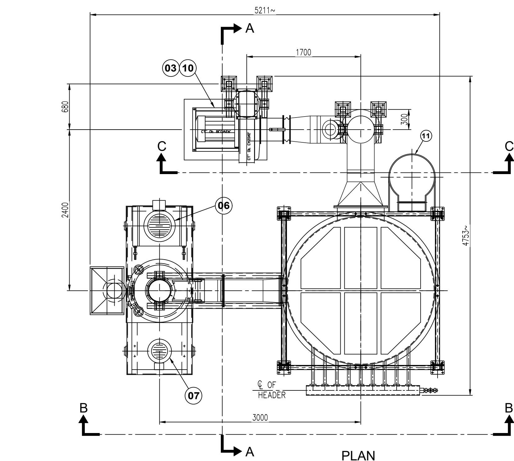
PLAN
