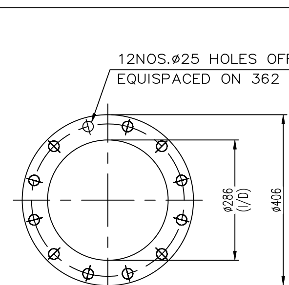
DETAIL-X RAL DISCHARGE FLANGE AL-250
